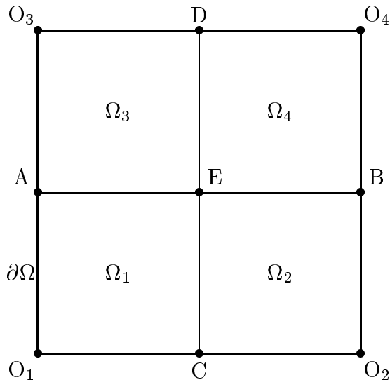
Fig. 5.1. A simple example with four subdomains.
